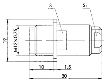
Instrument cable socket CP-50-154FB (See table 7)
