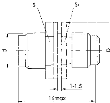
Threaded connection straight adapter (Needle- Needle)
