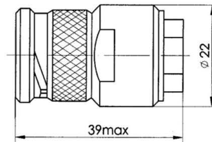
Bayonet connection straight cable plug
