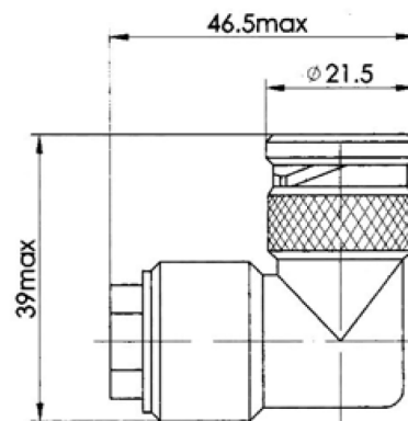
Bayonet connection elbow cable plug
