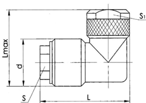
Threaded connection elbow cable plug (See table 3)
