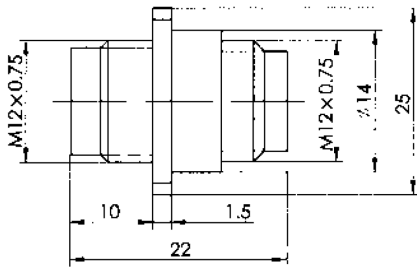
Unsealed adapter CP-50-160FB
