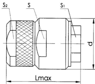
Straight cable plug with threaded connection (See table 2)
