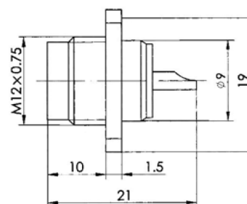
Instrument socket CP-50-150FB
