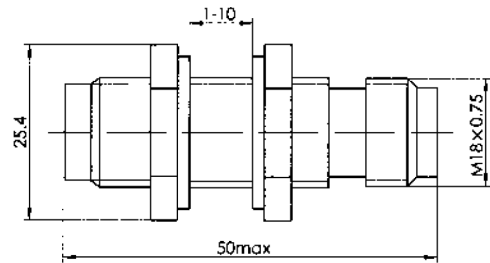
Threaded connection lower adapter (hole-hole)
