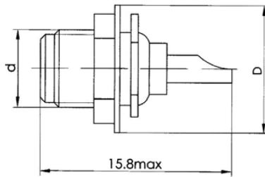
Threaded connection socket CP-50-267FB (See table 1) CP-75-268FB
