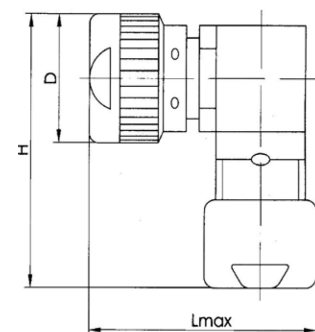
Elbow plug CP-50-287FB (See table 4)
