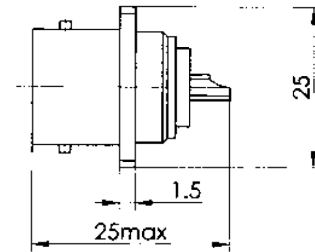
Bayonet connection socket CP-50-65FB CP-75-66FB
