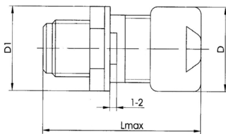
Straight socket CP-50-282FB (See table 5)
