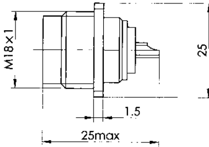
Threaded connection socket CP-50-165FB
