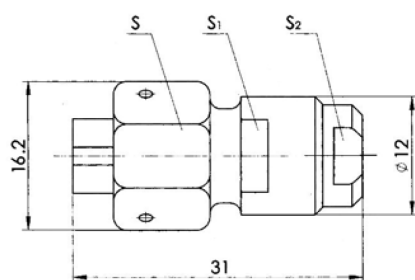
Straight cable plug (See table 6)
