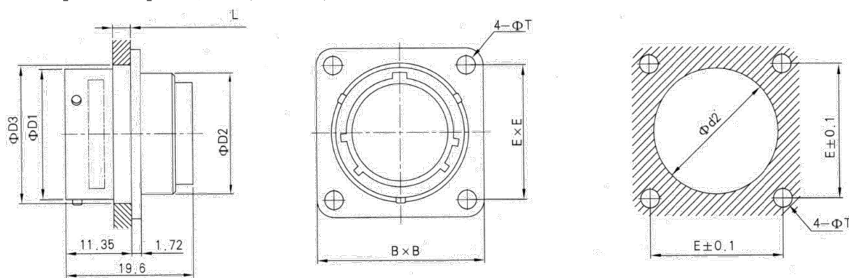
Box square receptacle, rear (RF27508)
