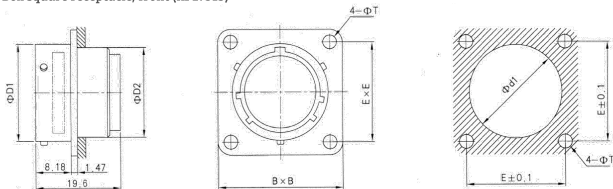
Box square receptacle, rear (RF27508)
